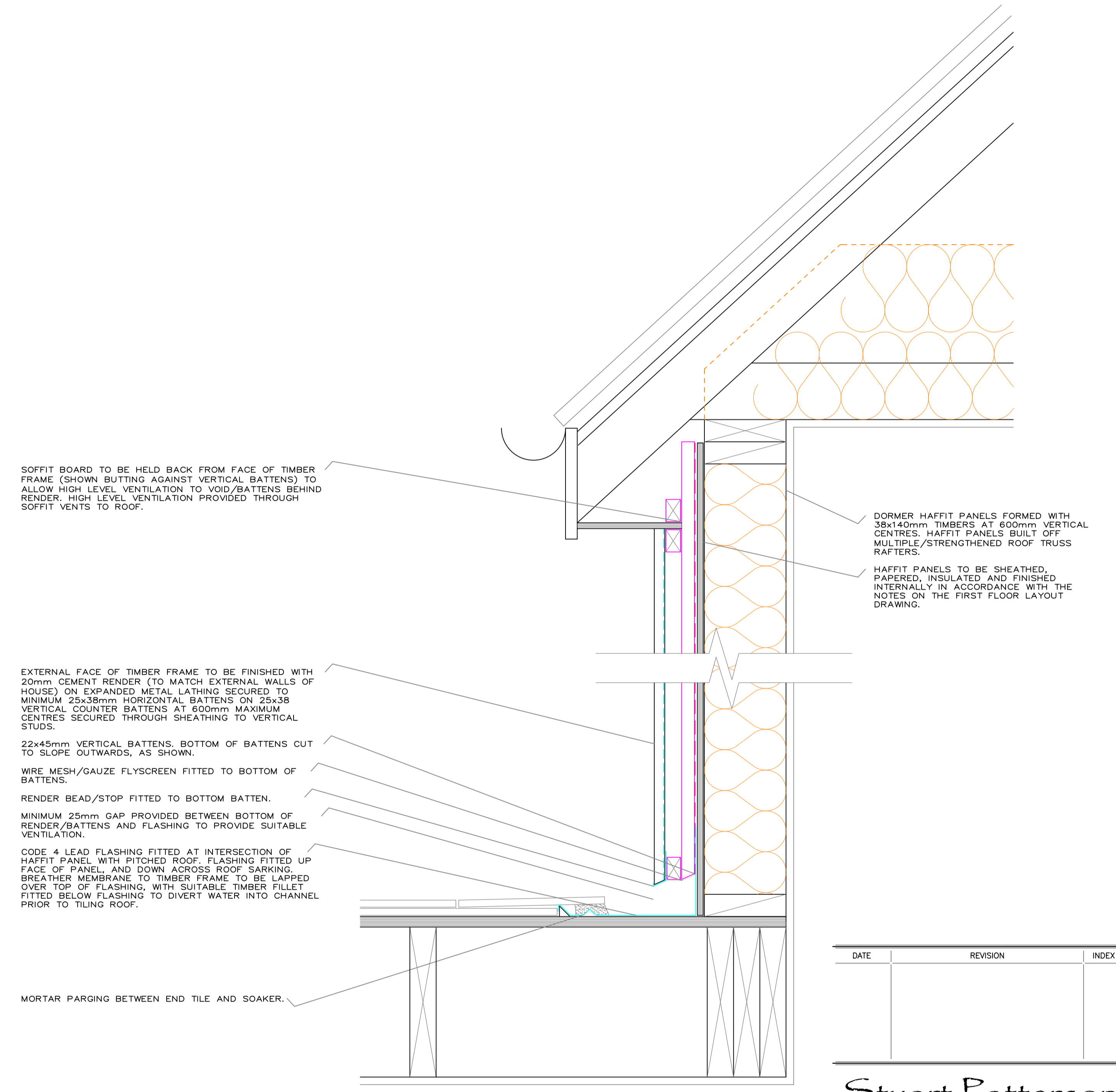
Detail Through Haffit Infill Panels SCALE 1:5.
